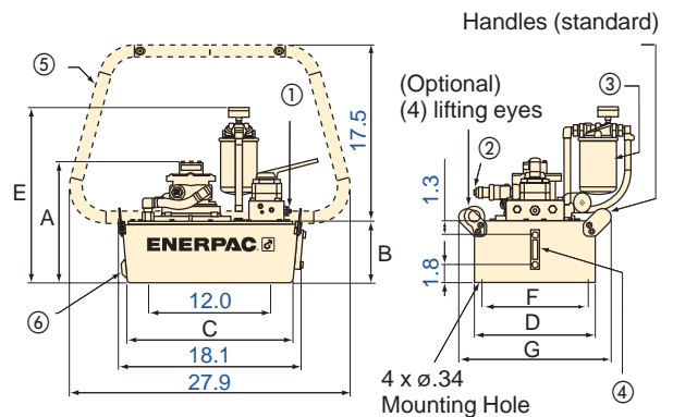
2.5, 5, 10 gallon reservoirs
