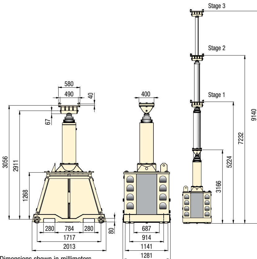
Dimensions shown in millimeters.
